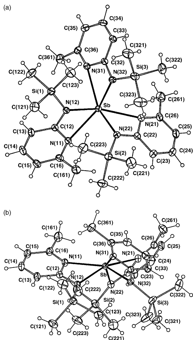
Fig. 3 Molecular projection of [\{2-(6\text{-Me})\text{C}_5\text{H}_3\text{N}\}\text{NSiMe}_3]_3\text{Sb} , (4) (( 5 ) is isostructural) projected down (a) and normal to (b) the non-crystallographic C_3 axis, showing atom labelling scheme.
