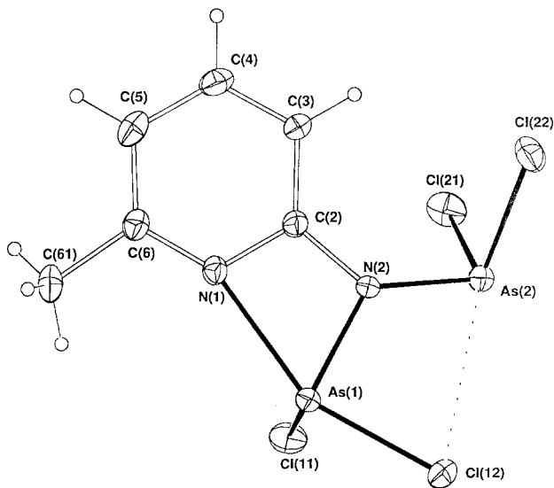
Fig. 2 Molecular projection of [2-(6\text{-Me})\text{C}_5\text{H}_3\text{N}]\text{N}(\text{AsCl}_2)_2 , (3), showing atom labelling scheme.
