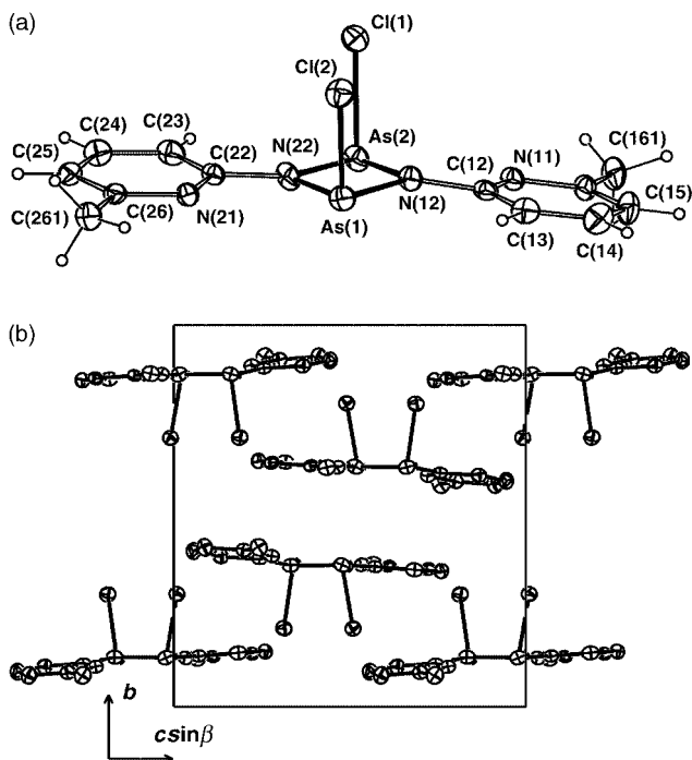
Fig. 1 (a) Molecular projection of [2-(6\text{-Me})\text{C}_5\text{H}_3\text{N}]\text{NAsCl}_2 , (2), showing atom labelling scheme. Non-hydrogen thermal ellipsoids are drawn at the 20% probability level here and in subsequent figures, hydrogen atoms having arbitrary radii of 0.1 Å. (b) The unit cell of (2) projected down a .
